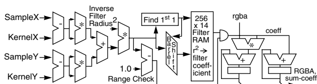
Figure 3: Filter Processor Detail.
